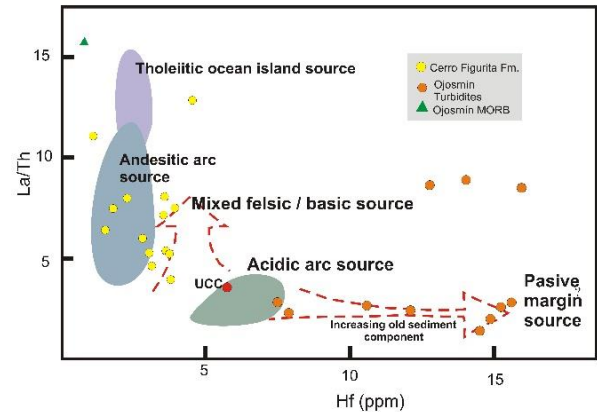
Figure 16. La/Th vs Hf discriminant diagram after Floyd and Leveridge (35) illustrating the radical change in provenance from a relatively unrecycled CFFm to an extremely reworked sediment for OU turbidites
