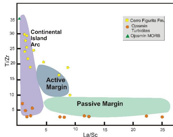
Figure 15. La/Sc vs. Ti/Zr discriminant diagram plot tectonic setting, after Bhatia and Crook (34)
