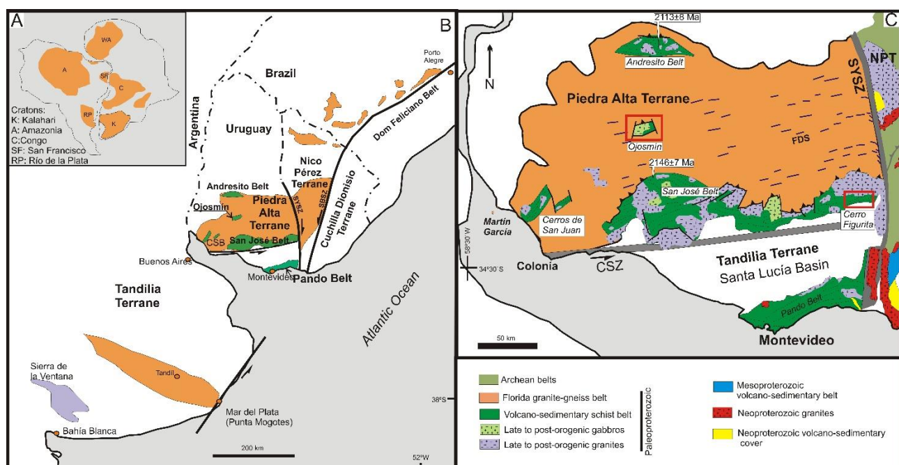
Figure 1. A: Location of the Río de la Plata Craton. B: and C: Piedra Alta Terrane in Uruguay Bossi and Cingolani (3) . CSZ: Colonia Shear Zone, NPT: Nico Pérez Terrane, FDS: Florida Dike Swarm, SYSZ: Sarandí del Yí Shear Zone
