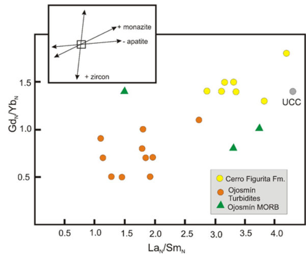
Figure 12. \text{Gd}_N/\text{Yb}_N vs. \text{La}_N/\text{Sm}_N after Bock and others (47) shows a vertical trend in the OU sample set, which is related to the effect of zircon addition
