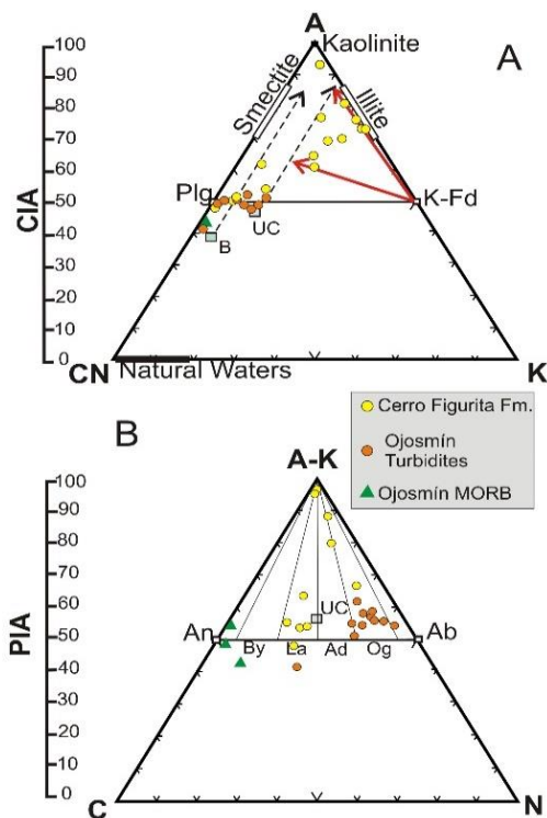
Figure 10. Chemical alteration of the analyzed rocks. A) Ternary A-CN-K ( \text{Al}_2\text{O}_3 -[ \text{CaO}^*+\text{Na}_2\text{O} ]- \text{K}_2\text{O} ) diagram; arrow-headed lines indicate normally predicted weathering trend (41) of average post-Archaean Upper Continental Crust (empty square denotes UCC and B unaltered basalt). The spread of the data indicate composition range from granodiorite to basalt. B) Ternary AK-C-N ( \text{Al}_2\text{O}_3+\text{K}_2\text{O} )- \text{CaO}^* - \text{Na}_2\text{O} . CIA: Chemical Index of Alteration. Note that most samples of Ojosmín turbidites plot in the bulk oligoclase field. PIA: Plagioclase Index of Alteration. An=anorthite, By=bytownite, La=labradorite, Ad=andesine, Og=oligoclase, Ab=albite
