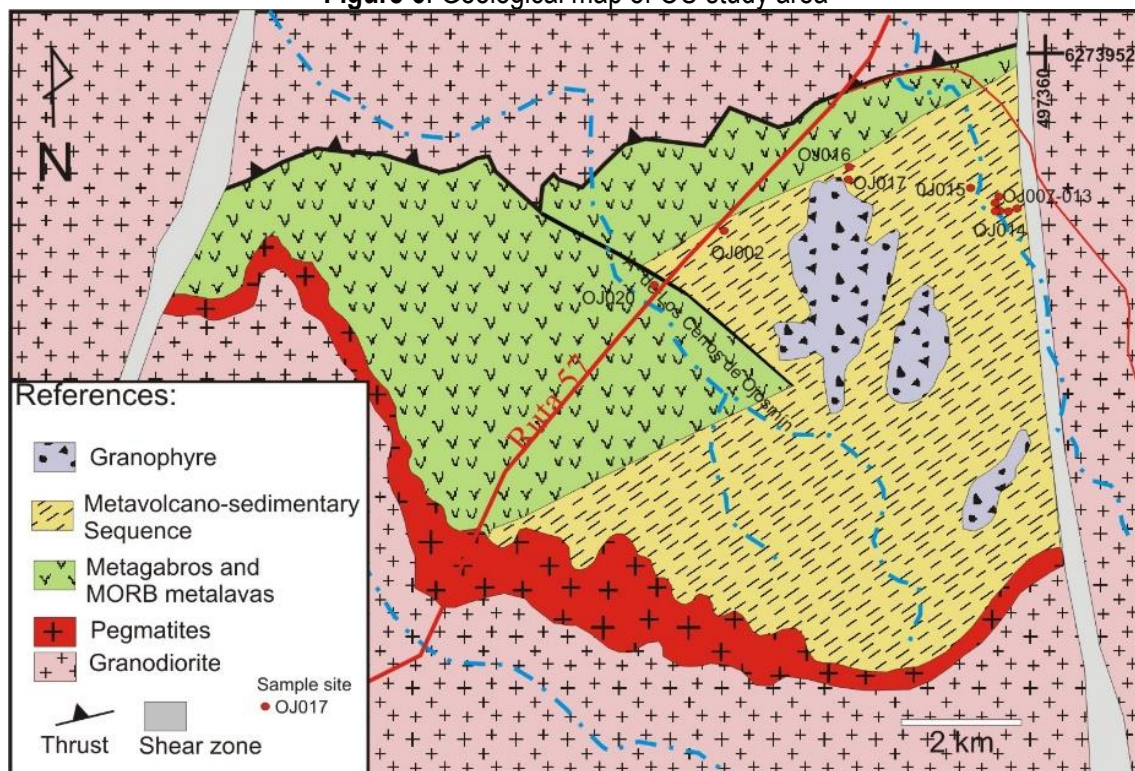
Figure 6. Geological map of OU study area
