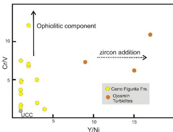
Figure 14. Cr/V vs. Y/Ni diagram Hiscott (48) shows the ophiolitic source rock component of CFFm and Y enrichment of Ojosmin turbidites due to zircon addition
