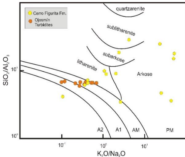
Figure 7. \text{K}_2\text{O}/\text{Na}_2\text{O}-\text{SiO}_2/\text{Al}_2\text{O}_3 after Roser and Korsh (31) and Pettijohn and Potter (32) . PM: passive Margin, AM: active margin, A1: arc setting, A2: evolved arc setting
