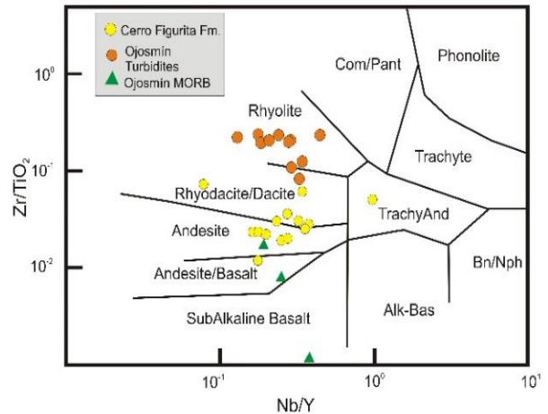
Figure 8. Nb/Y-Zr/TiO 2 diagram after Winchester and Floyd (37)
