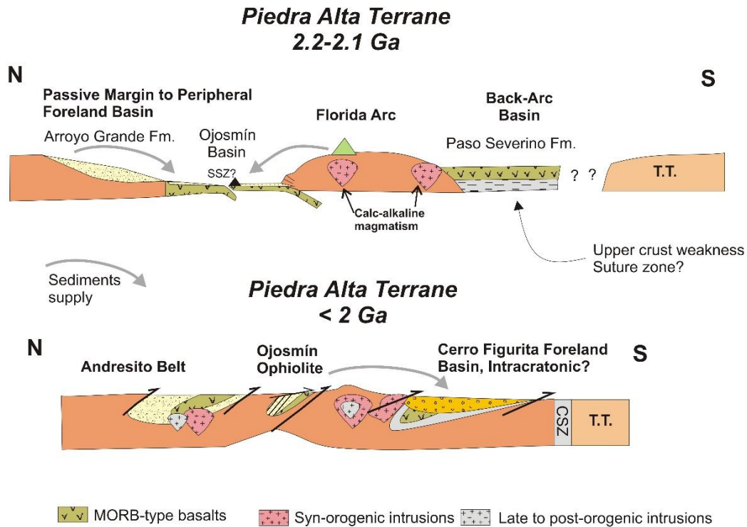
Figure. 17. Sketch representing the paleogeographic evolution and the main source areas during the deposition of the OU and the CFFm during the Paleoproterozoic. T.T.: Tandilia Terrane, SSZ: Suprasubduction Zone, CSZ: Colonia Shear Zone
