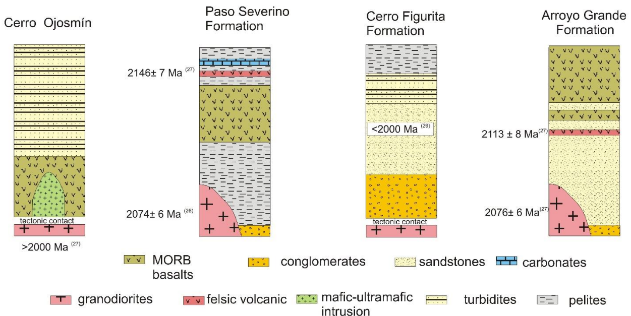
Figure 2. Comparison between key meta(volcanic)sedimentary sequence of the Piedra Alta Terrane and their main stratigraphic features from Bossi & Piñeyro (29) and Blanco and others (30)
