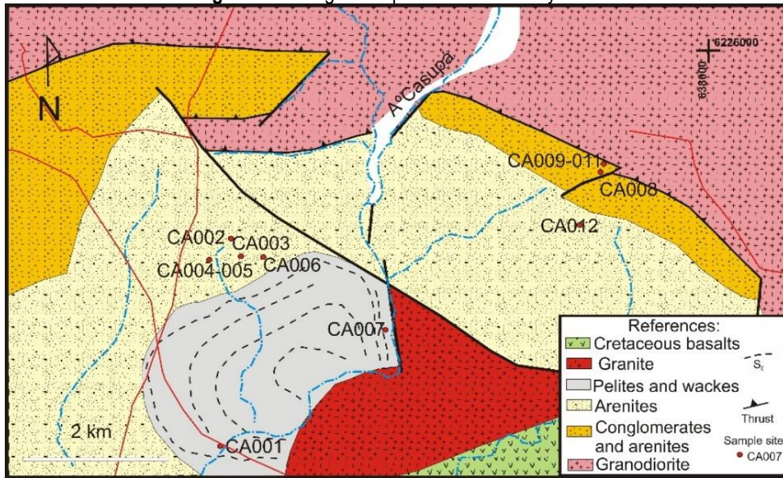
Figure 4. Geological map of the CFFm study area
