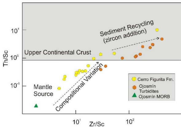
Figure 13. Th/Sc vs. Zr/Sc diagram (39) . Discussion in the text
