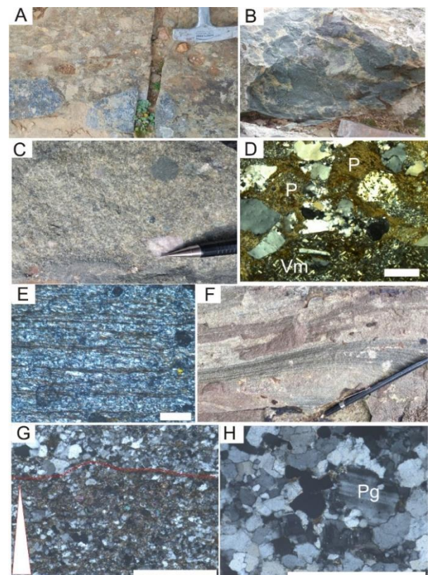
Figure 5. Outcrops and thin sections of the CFFm: A) coarse polymictic conglomerate; B) volcanoclastic breccia; C) conglomeratic sandstones; D) detrital pelite (P), and volcanic clasts (Vm) in a lithic arenite; E) alternation of detrital quartz-feldspar and illite-chlorite laminae, turbiditic facies. OU: F) sandstone outcrop; G) normal grading in turbiditic sandstones; H) albitized plagioclase in fine sandstone showing concave-convex grain contacts. Scale bar represents 200 \mu m
